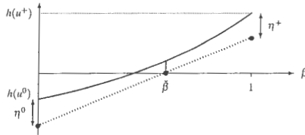
Fig. 1 Interpolation guarantees h(\tilde{u}) \leq (1 - \tilde{\beta})\eta^0 + \tilde{\beta}\eta^+
