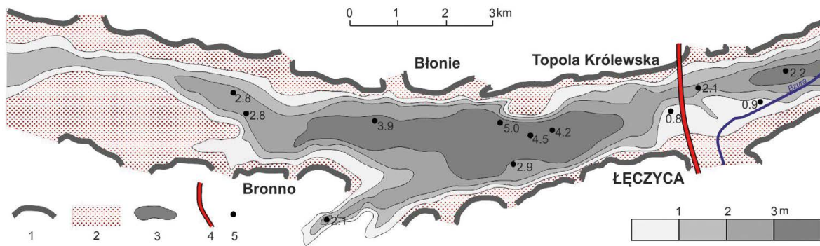
Figure 4. Peat thicknesses in the Warsaw-Berlin ice-marginal spillway (Bzura-Ner valley section) near Łęczycza (after Domosławska-Baraniecka, 1968). 1 – edges of the valley, 2 – range of river sands, 3 – peat isolines (every 1 m), 4 – embankment of road (DK 91), 5 – selected boreholes, confirmed peat thicknesses
