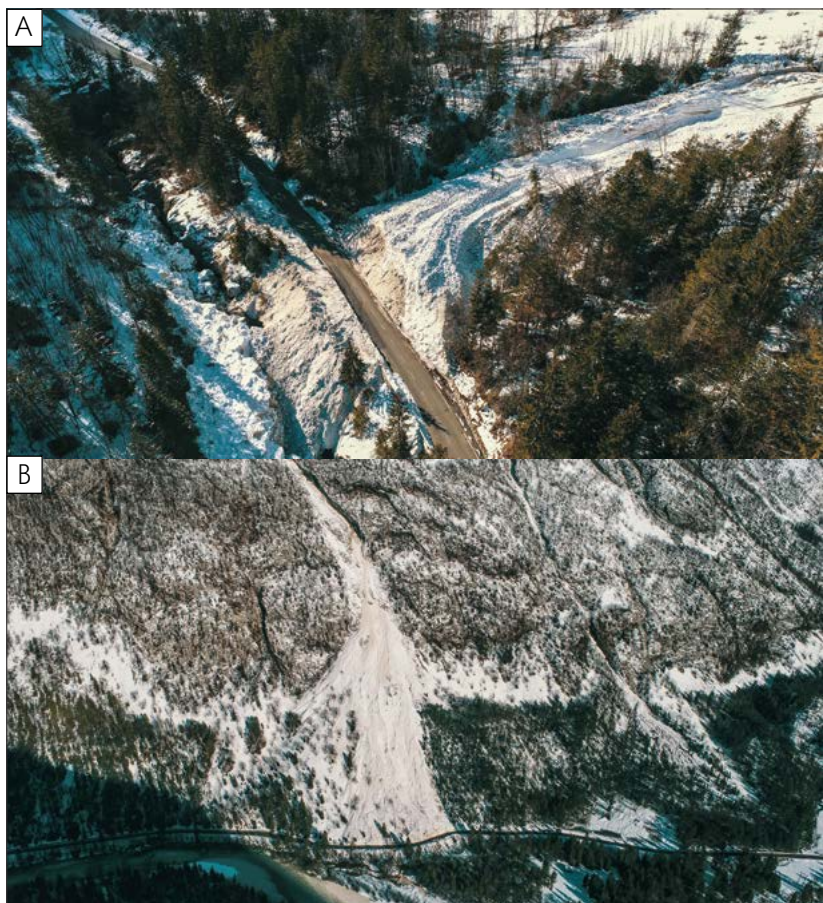
Figure 9. (A) The V Koritih avalanche reached the valley floor and partially buried Great Soča Troughs, left of the road (Photo by Jure Tičar; GIAM ZRC SAZU Archives, 2021). (B) The Širokec avalanche moved to the less vegetated, eastern part of the scree (Photo by Jure Tičar; GIAM ZRC SAZU Archives, 2021)
