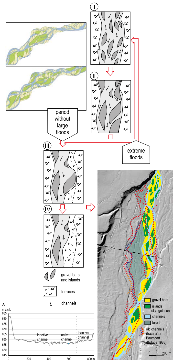
Figure 7. Conceptual model of braided river development experiencing degradation on the example of the Białka river channel; Degradation of the braided reaches of the Białka River (reach 8, river channel from the 1980s, based on Baumgart-Kotarba, 1983a,b)
