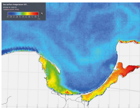
Figure 8. Spatial features of surface water temperature of the Gdańsk Bay on 16.04.2019 in accordance with the site http://satbatyk.iopan.gda.pl (data provided by System SatBaTyk)
