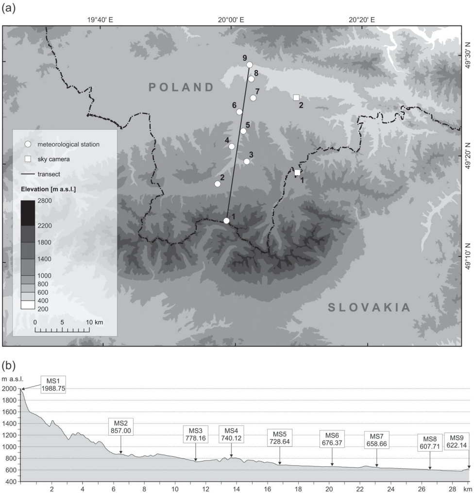
Figure 1. The orography of the Tatra Mountains with locations of the meteorological stations (MSs) and sky cameras (a) and transect of terrain Kasprowy Wierch (MS1) – Nowy Targ (MS9) with approximate locations of MSs 2-8 (b) (numbers in boxes indicate height above sea level of the barometers at each station)
