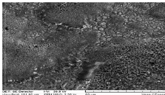
Fig.2. An example of the surface of C45 steel following diffusion chromizing and laser heat treatment, variant no 1, SEM
