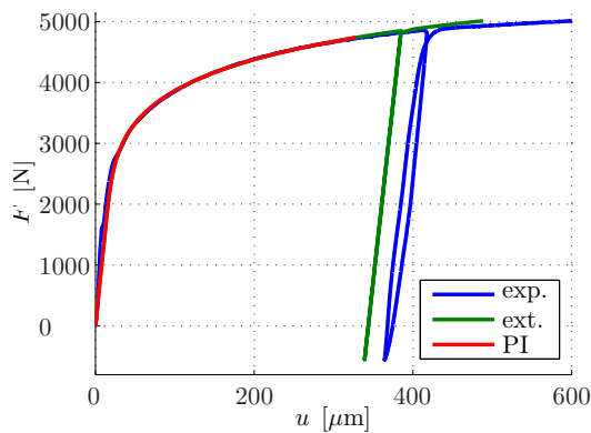
Figure 1: Load displacement diagram of the tension test including unloading underlying the PI. Experiment (blue), PI result (red) and simulation including the unloading (green).
