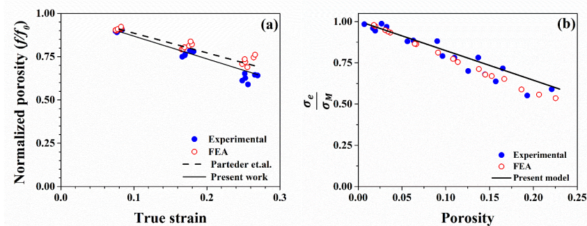
Fig. 1: (a) Comparison of experimental, FEA and theoretical results for normalized porosity ( f/f_0 ) during compression (b) Variation in normalized flow stress ( \sigma_e/\sigma_M ) with porosity, comparison between experimental data, FEA predictions and theoretical analysis
