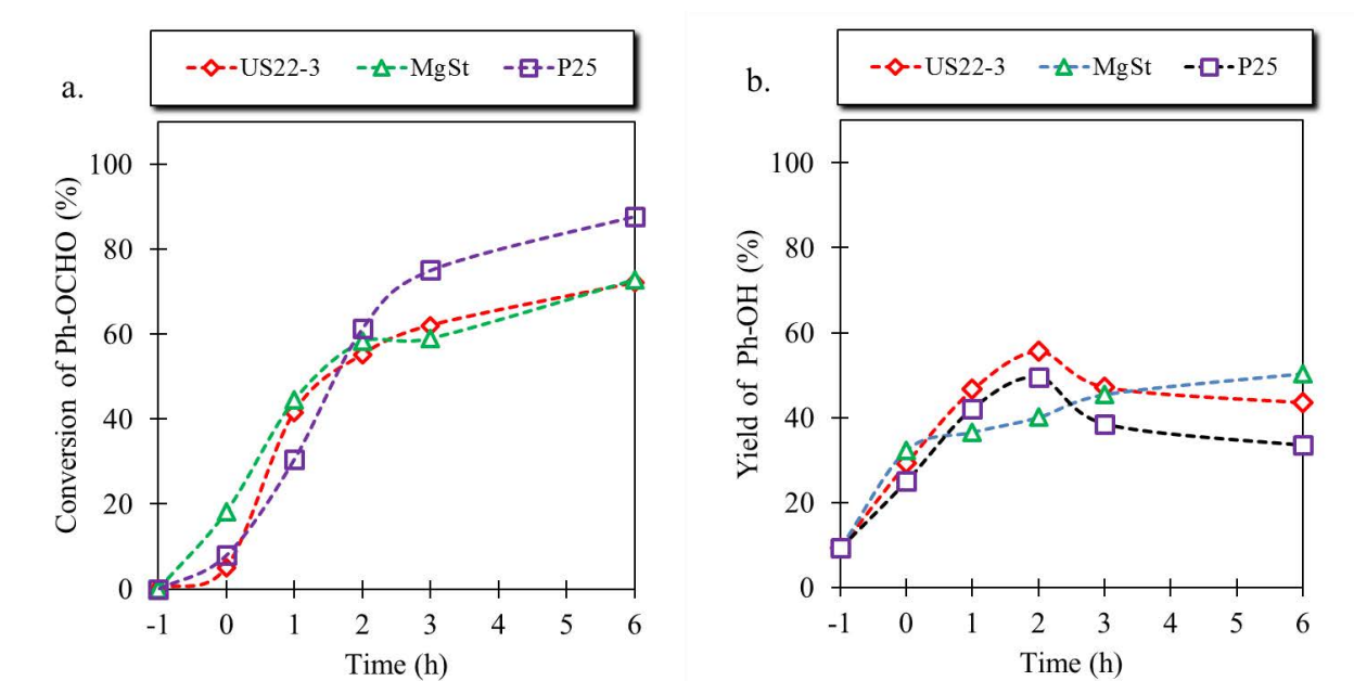
Figure 4.36. Photocatalytic activity of 22kHz-3, MgSt and P25 samples for the conversion of Ph-OCHO (a), yield of Ph-OH (b). (Based on the results of the article submitted to ACS Sustainable Chemistry and Engineering)
