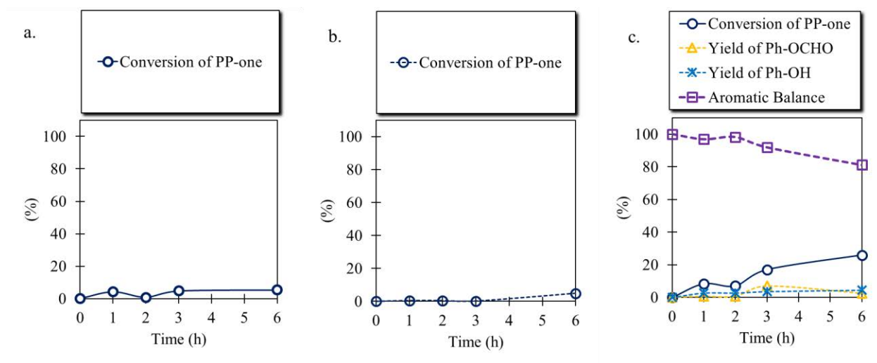
Figure 4.35. Photocatalytic conversion of PP-one by using samples 22kHz-3 (a), MgSt (b) and P25 (c). (Based on the results of the article submitted to ACS Sustainable Chemistry and Engineering)
