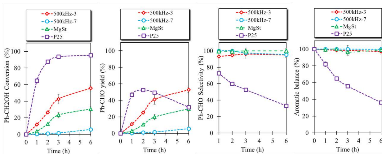
Figure 4.25. Photocatalytic activity of 500kHz-3, 500kHz-7, MgSt, and P25 samples for partial selective oxidation of Ph-CH 2 OH to Ph-CHO. (Based on the results published in open access article [123])
