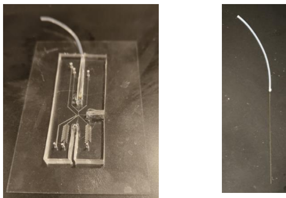
Figure A1.5: Shows the final device with the glass capillary inserted and fixed. On the right, the glass capillary (inner diameter: 40 \mu\text{m} ) is glued to the tubing.
