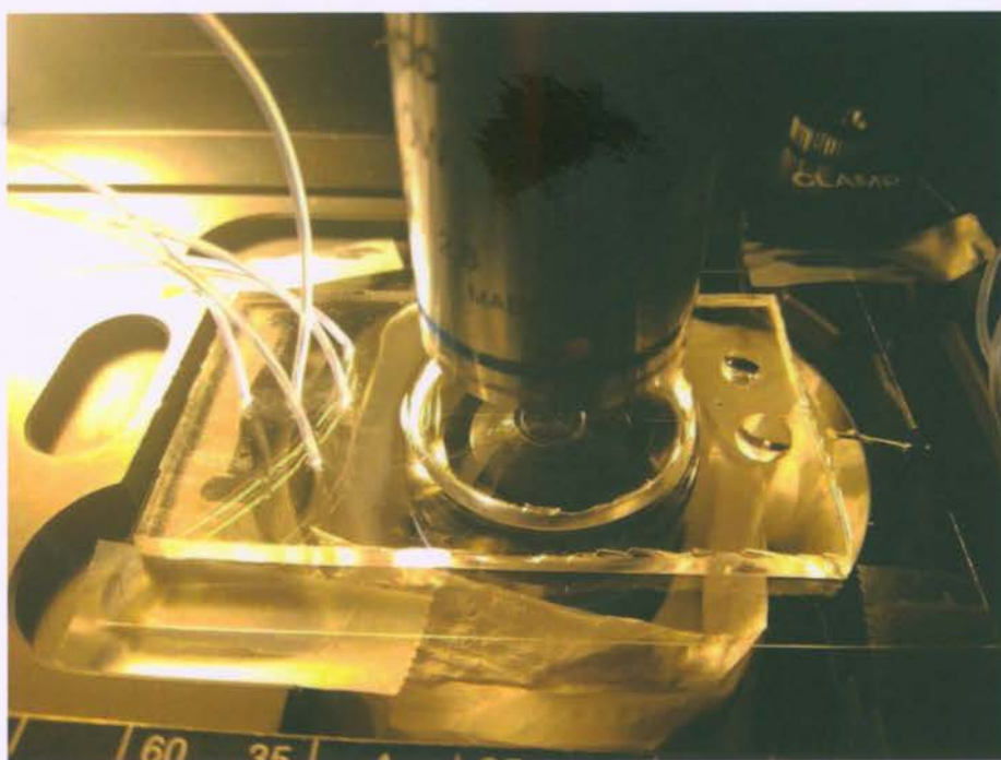
Photograph of the microfluidic device integrated with a Raman microscope, employed for imaging single cells.
