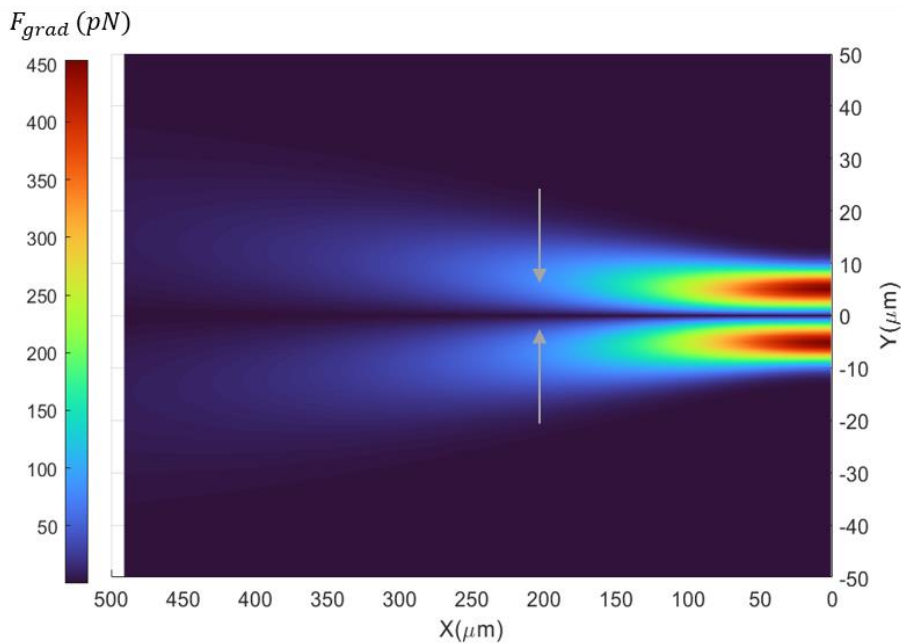
Figure 29: The gradient force exerted by the laser beam from an optical fiber on a 15 \mu\text{m} PS bead flowing in the microfluidic channel.
