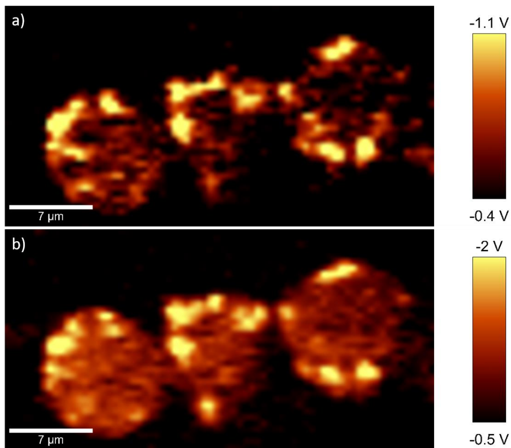
Figure 48: TOM-1 cells incubated in OA imaged at (a) 2,850\text{ cm}^{-1} and (b) 2,930\text{ cm}^{-1} . Scale bars corresponding to 7\text{ }\mu\text{m} .
