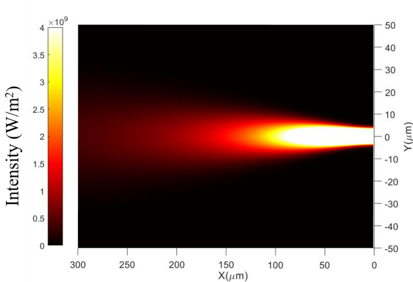
Figure 23: Beam profile visualised within the channel as a result of scattering due to 500 nm PS particles.
