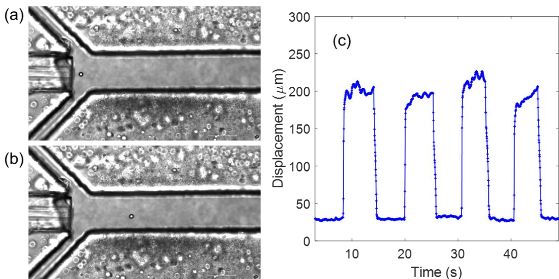
Figure 31: Microscopic image depicting a trapped PS bead of diameter 15 \mu\text{m} at a laser power of (a) 182 mW and (b) 500 mW for a fixed flow velocity. (c) The relative change in the X-position of the particle is measured by manipulating the particle between two positions by modulating the laser powers.
