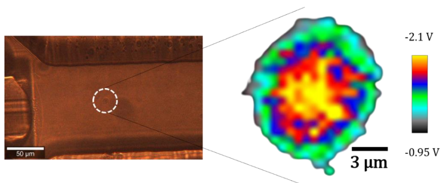
Figure 44: Spatial distribution of the proteins of a trapped cell obtained by stimulated Raman imaging at 2,940 \text{ cm}^{-1} . The intensity of the SRS signal is depicted on the colour scale (190).
