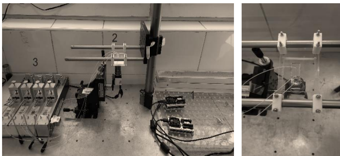
Figure A2.2: Components of the setup for the tweezing experiments 1. Fiberized laser diodes 2. Chip assembly (also shown on the right). 3. Cetoni syringe pumps for flow actuation.
