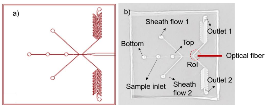
Figure 16: (a) AutoCAD design of the microfluidic chip. (b) The corresponding PDMS chip after fabrication is bonded on glass.
