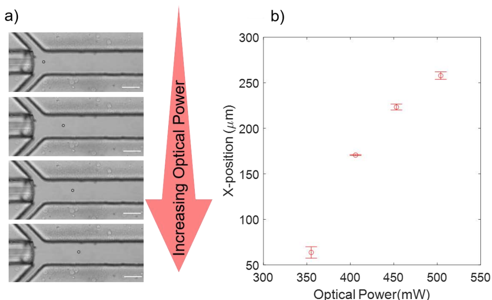
Figure 36: Translation of a trapped 15 \mu\text{m} PS particle while varying the applied laser power at the output end of the fiber and maintaining a constant flow velocity of 600 \mu\text{m/s} in the microchannel.
