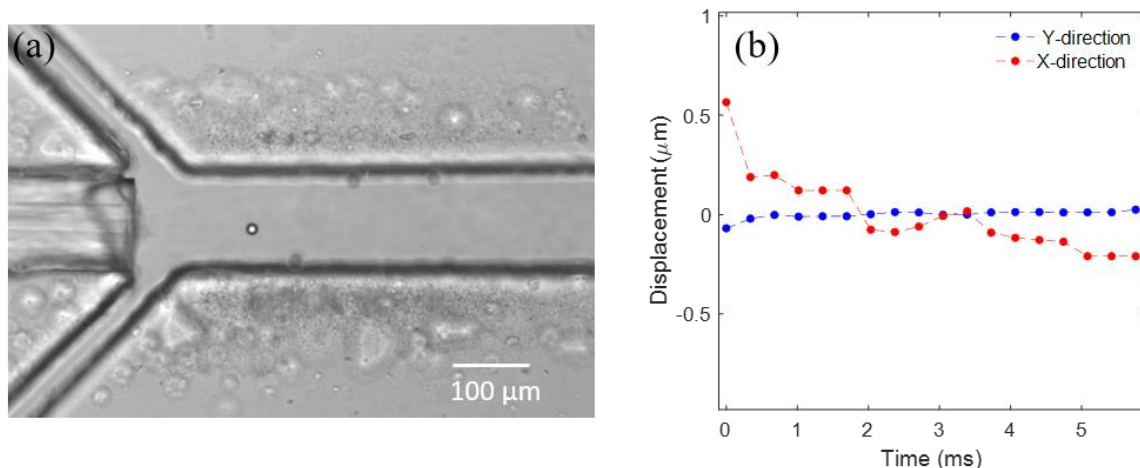
Figure 30: (a) Microscopic image of a 15 \mu\text{m} PS bead trapped in the microchannel using OHT. (b) Fluctuations around the mean position of the trapped bead in the X- and Y- directions. The position corresponds to the centroid coordinates of the particle extracted from individual frames.
