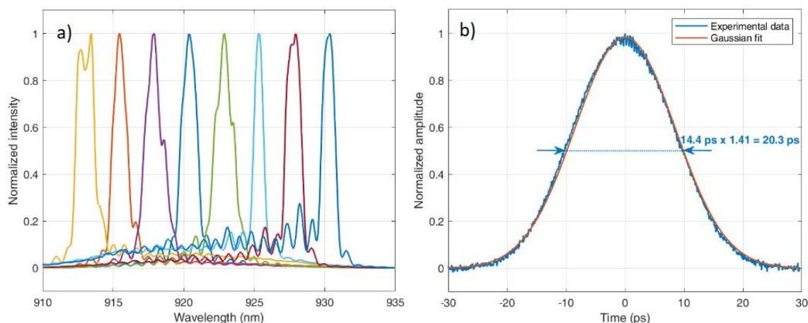
Figure 5.10: a) Tunable pump spectra with an average power of 50 mW for each spectrum. b) Pulse profile with a temporal duration of 14.4 ps measured for a selected pump beam at 920 nm.
