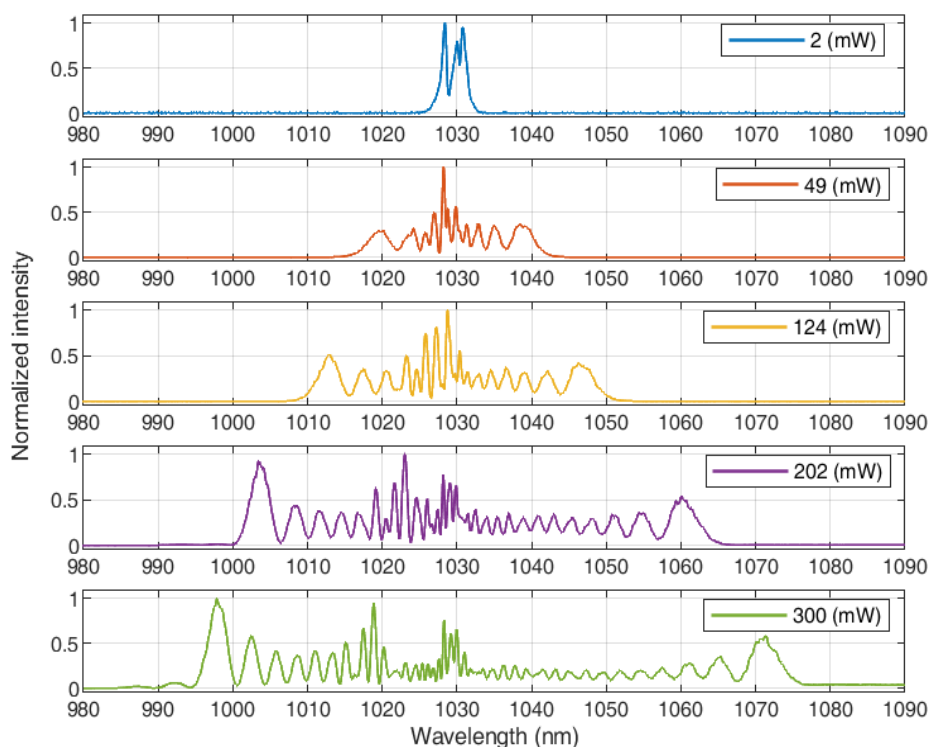
Figure 5.12: SPM evolution as a function of the pump power.
