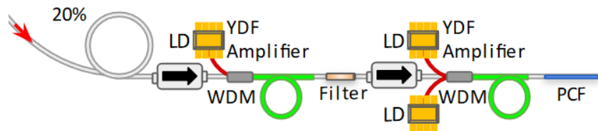
Figure 5.11: Schematic of the spectrum broadening.
