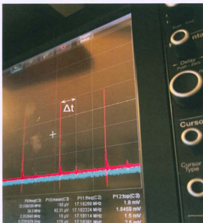
Figure B.1: Synchronization between the cavities using the oscilloscope.
