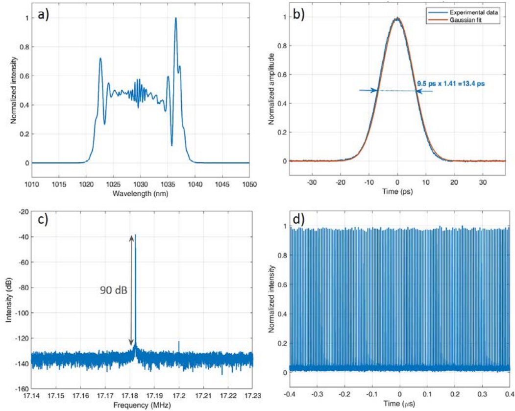
Figure 5.3: a) Output spectrum centered at 1030 nm with an FWHM of 14 nm and b) pulse profile with a temporal duration of 9.5 ps. c) Radio-frequency (RF) spectrum of the generated output pulse train centered at 17.18 MHz and d) output pulse train, fluctuations are caused by the undersampling of the oscilloscope.
