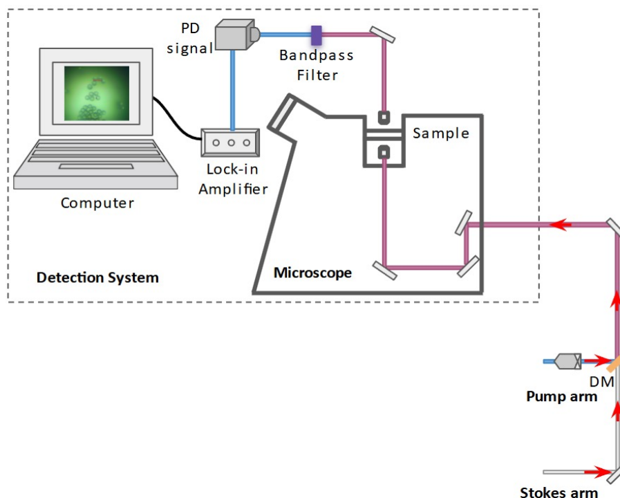
Figure 5.16: Detection system based on lock-in amplifier.
