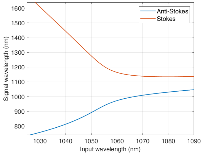
Figure 6.2: Calculated phase-matching diagram of anti-Stokes (blue) and Stokes (red).
