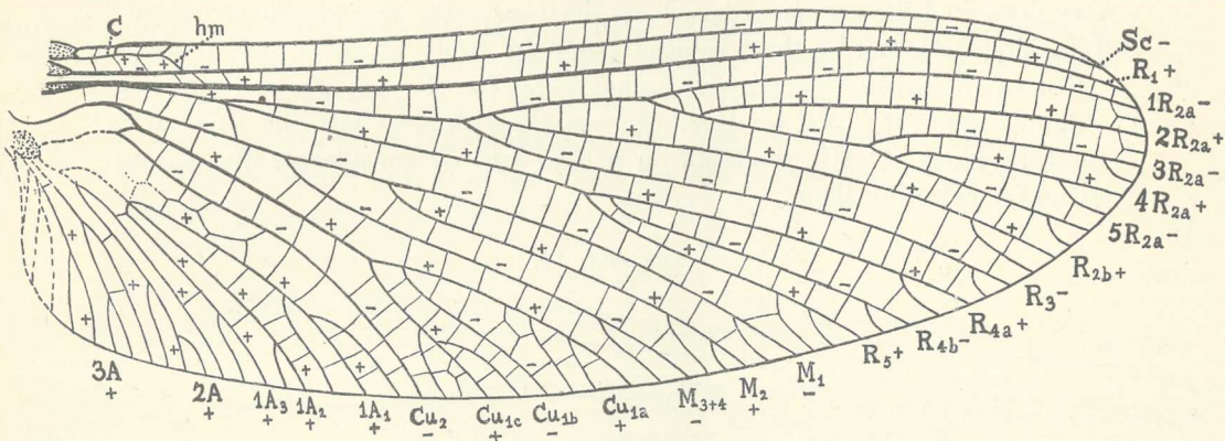
Hind-wing of Protereisma sp., Lower Permian of Kansas; the fore-wing is closely similar, but a little narrower at base, as shown in text-fig. 3.
