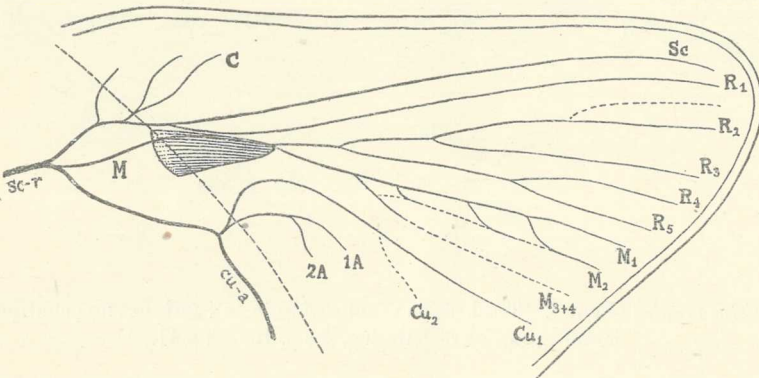
Ameletus ornatus (Eaton). Tracheation of fore-wing in (n+1) th larval instar. For lettering, see p. 162. ( \times 87 .)
