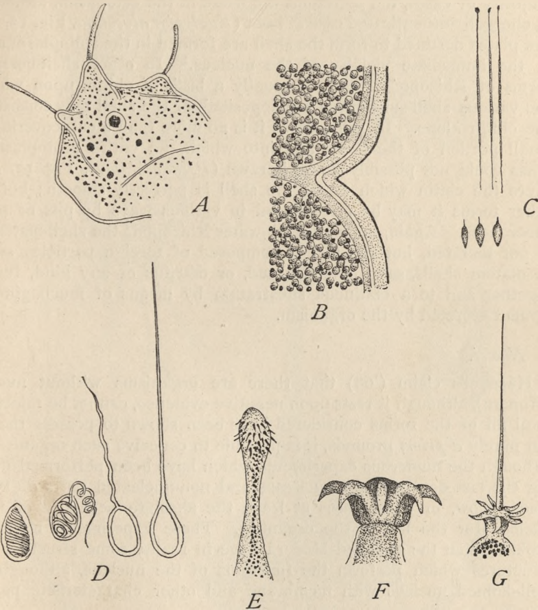
Fig. 12. — Ectoplasmic modifications.
