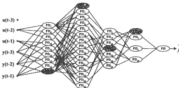
Fig. 14. Optimal modified PNN structure in Type II (2→3 node inputs and Type 1→Type 2)
