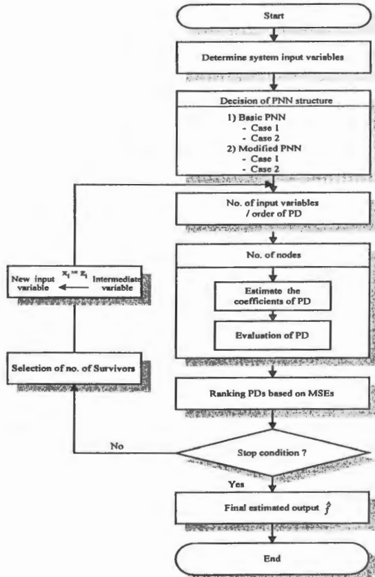
Fig. 2. Flowchart of the PNN algorithm
