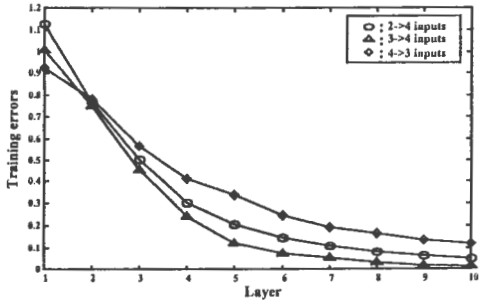
Fig. 20. Performance index for the training data (Type 1→Type 2)
