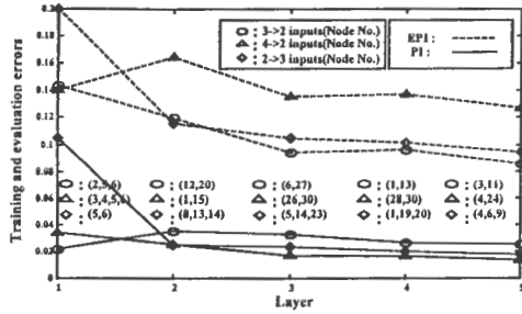
Fig. 11. Performance index for training and evaluation in Type II (every layer: Type 2)
