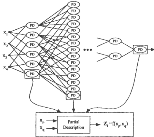
Fig. 3. Configuration of the basic PNN structure - Case 1
