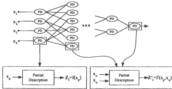
Fig. 6. Configuration of the modified PNN structure – Case 2
