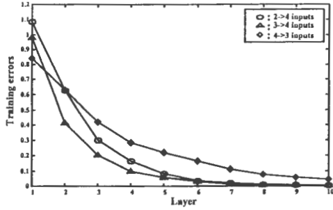
Fig. 19. Performance index for the training data (each layer is of Type 2)
