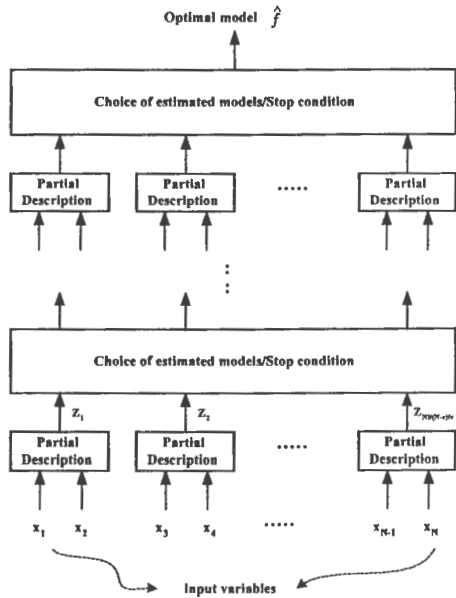
Fig. 1. An overall architecture of the PNN
