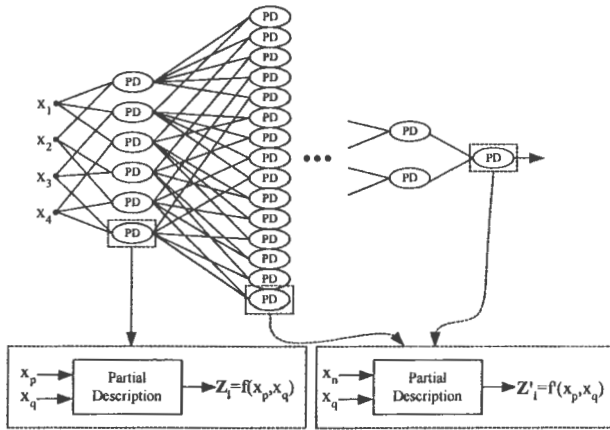
Fig. 4. Configuration of the basic PNN structure – Case 2.
