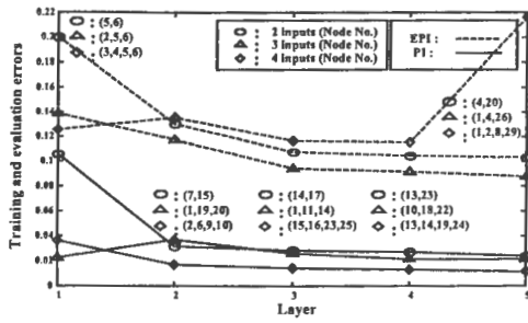
Fig. 9. Performance index for training and testing in Type II network (Type 1 → Type 2)
