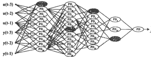
Fig. 10. Optimal PNN structure of Type II (3 inputs and Type 1 → Type 2)
