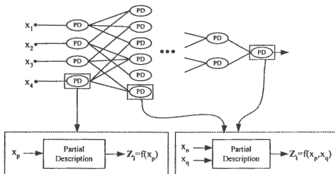
Fig. 5. Configuration of the modified PNN structure – Case 1.
