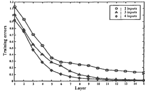
Fig. 18. Performance index for the training data( Type 1→Type 2)
