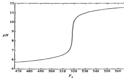
Fig. 16. Titration curve for pH neutralization
