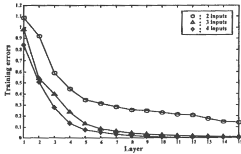
Fig. 17. Performance index for the training data (each layer is of Type 2)
