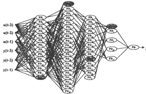
Fig. 8. Optimal PNN structure of Type II (4 inputs, Type 3); see description in text
