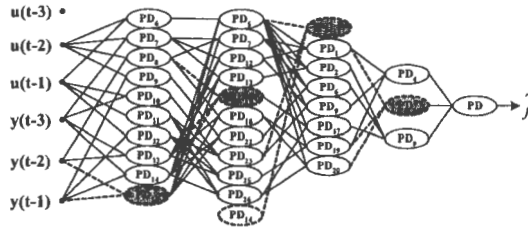
Fig. 12. Optimal modified PNN structure in Type II (Type 2 and 2→3 node inputs)
