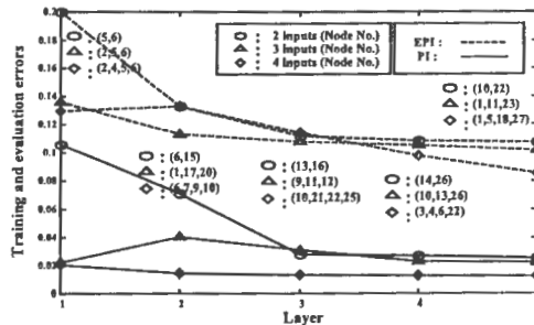
Fig. 7. Performance index for training and evaluation in Type II (each layer includes neurons of type 3)
