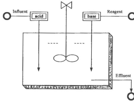
Fig. 15. A continuous tank reactor for pH neutralization
