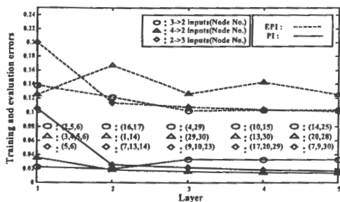
Fig. 13. Performance index for training and evaluation in Type II (1 st layer: Type 1, 2 nd layer or higher: Type 2)
