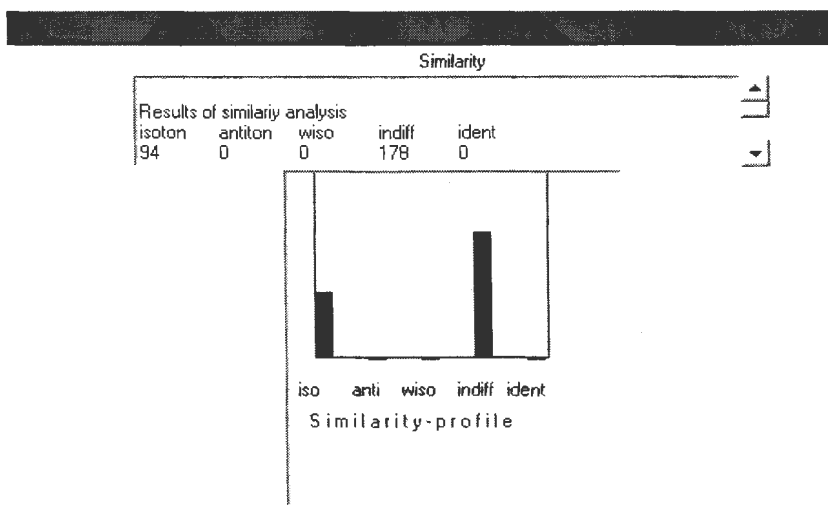
Figure 4. Results of similarity analysis of two data-sets (17x81 and 17x92) soil / needles
