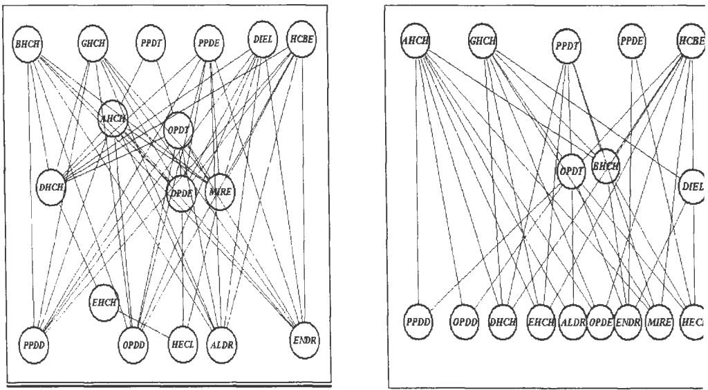
Figure 2. HD 17 pesticides x 81 soil samples (lhs) HD 17 pesticides x 92 needle samples (rhs)
