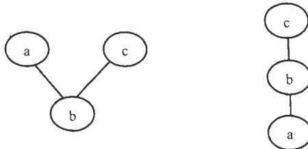
Figure 1. Two Hasse diagrams to demonstrate the similarity analysis
