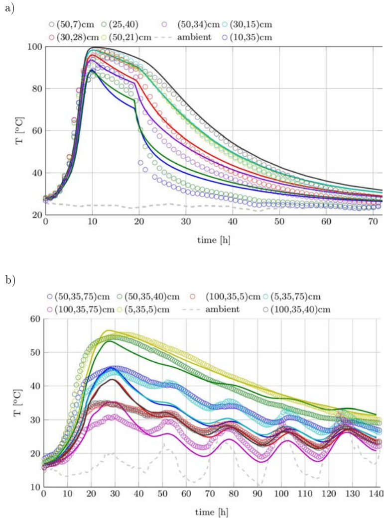
FIG. 5. Model validation: a) 2D case – mixture B, b) 3D case (cross-section) mixture A. Lines denote numerical solution, circles denote measurements.
