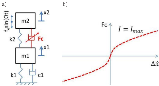
FIG. 1. a) The 2-DOF system layout, b) the force-velocity diagram of the MR damper.
