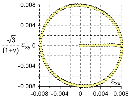
Fig. 1. Circular strain path for effective amplitude of ±0.8%
