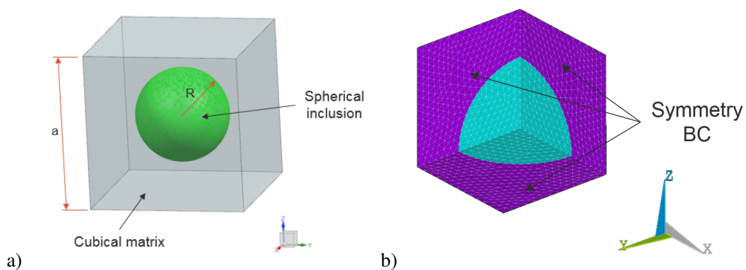
Figure 1: A composite unit cell (a) and its computational model analyzed in ANSYS. (b)
