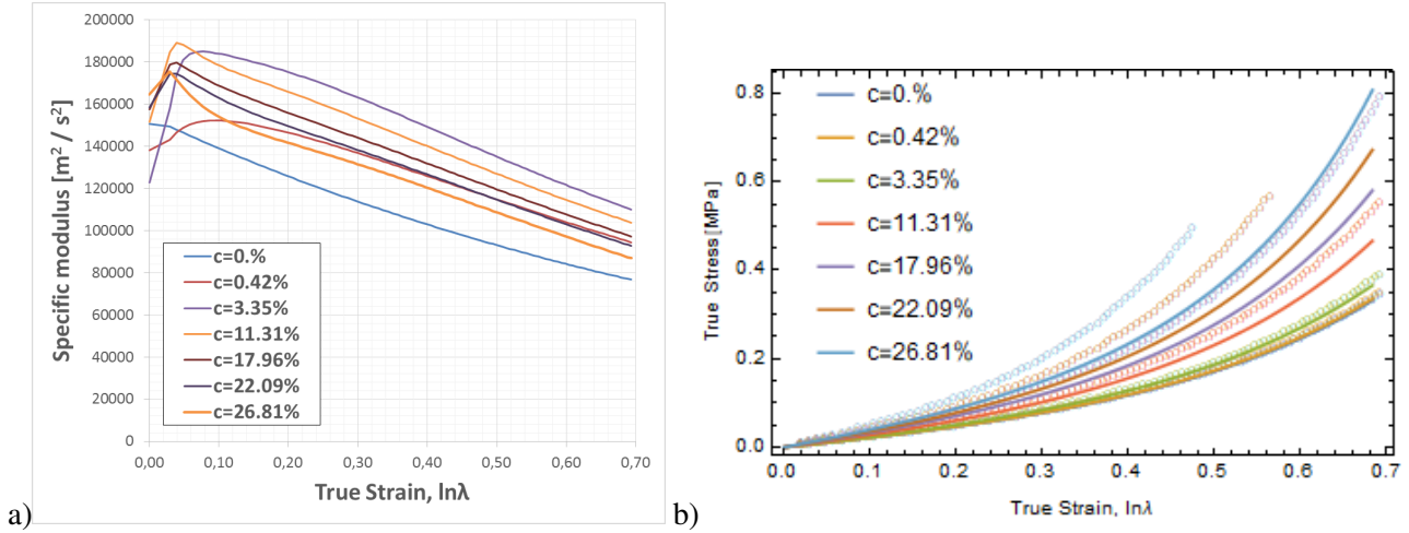
Figure 2: (a) Specific modulus as a function of true strain for steel matrix configuration (only FE analysis) (b) Comparison of true strain-true stress curves obtained by FE analyses (circles) and using micromechanical model (continuous line) for polymer matrix configuration.
