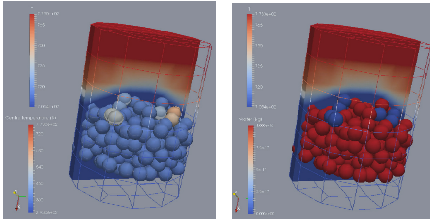
Figure 1: Temperature distribution and particle water content in a simplified reactor geometry
