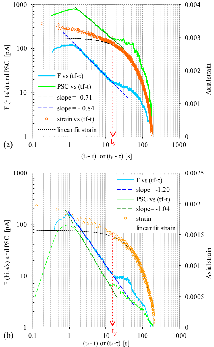
Figure 2: The PSC and the F-function against the (t_f - t) or (t_f - \tau) or parameters, in juxtaposition to the respective variation of the axial strain, for marble (a) and cement (b).
