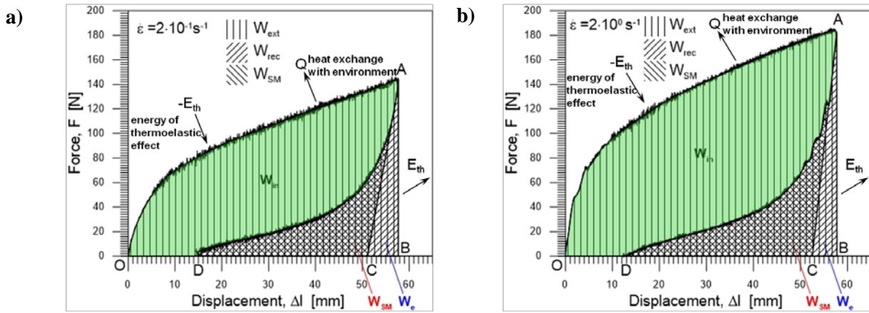
Figure 1: Scheme of energy estimation during PU-SMP loading-unloading cycle: a) 2 \cdot 10^{-1} \text{ s}^{-1} ; b) 2 \cdot 10^0 \text{ s}^{-1} .
