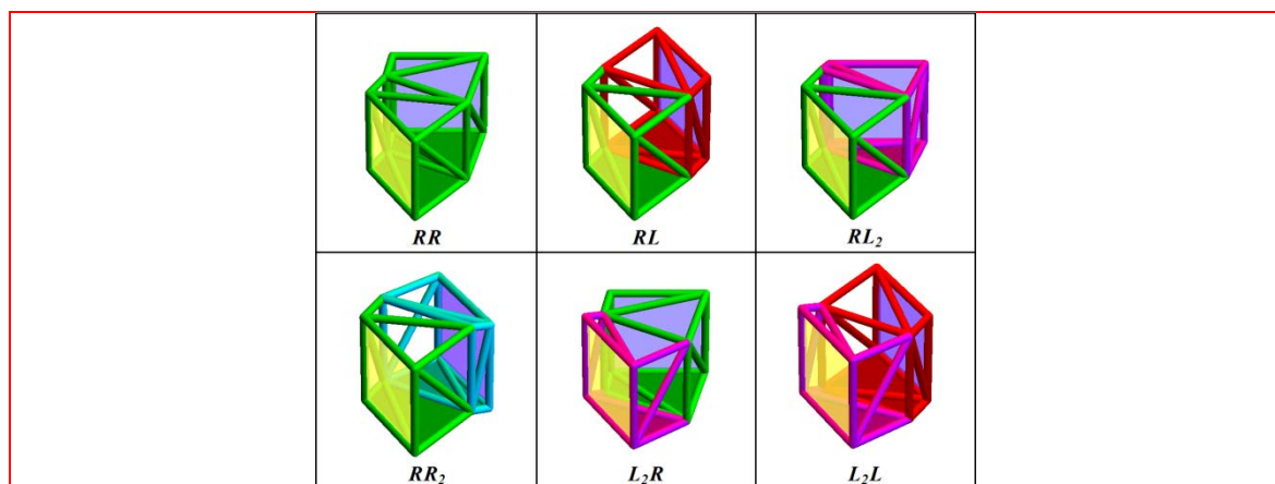
Fig. 5 The set S_2 of all essentially unique TZ structures of length 2. Module color convention as in Fig. 2. The fixing planes at the first and last module are indicated in: yellow and blue, respectively
