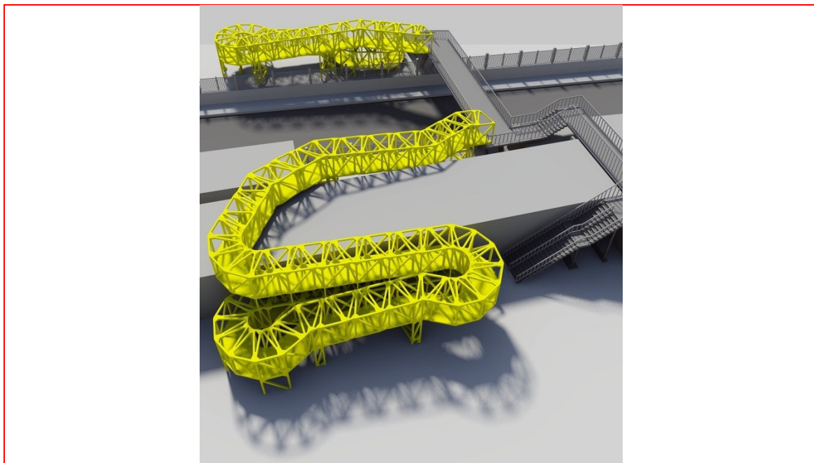
Fig. 3 Visualization of retrofitting of an existing overpass between two sections of Tokyo University Hongo Campus (Japan) with TZ (shown in yellow). Proposed gentle slope of the TZ ramp allows for safe crossing of elders, small children, wheel-chair users, persons with strollers, bicycles, etc. For further details on this case-study see Zawidzki (2015). Without the necessity of heavy equipment, TZ is a feasible solution for countless similar situations where pedestrian safety and comfort can and should be improved
