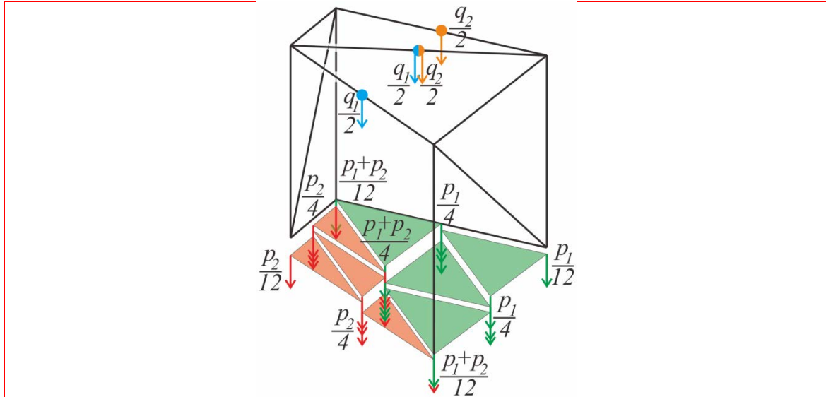
Fig. 7 Distribution of the static load used in the optimization process. The floor load ( p_1 + p_2 = 4000 \text{ N/m}^2 ) is allocated to the mid- and endpoints of the floor beams by treating the marked small congruent triangles as rigid. The ceiling load ( q_1 + q_2 = 1000 \text{ N/m}^2 ) is allocated to the midpoints of the horizontal beams in proportion to the area of the neighboring ceiling triangles
