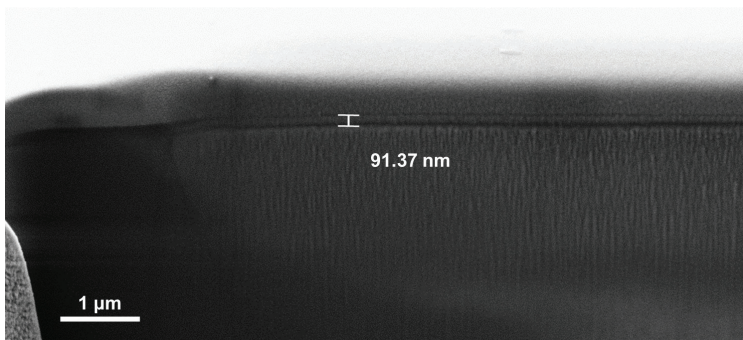
Fig. 9. SEM image of the FIB-etched section.
