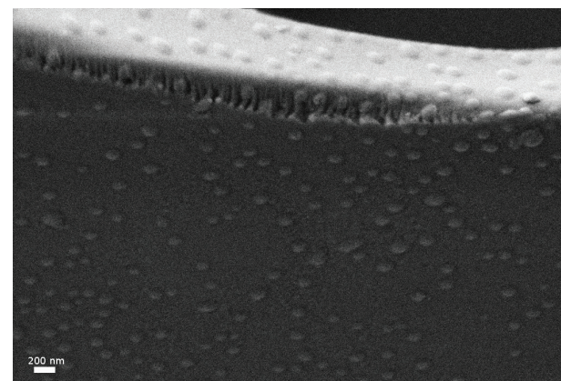
Fig. 6. \text{Al}_2\text{O}_3 layer visible on the surface of a broken sphere. The spots on the surface were identified as damage caused by the microscope electron beam, as they were appearing progressively with successive scans.
