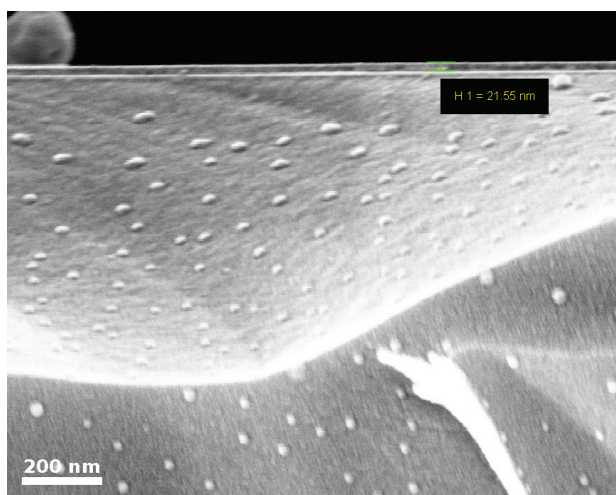
Fig. 3. SEM measurement of the \text{Al}_2\text{O}_3 layer on a fractured microscope slide after 200 deposition cycles. The imaging angle may cause a slight underestimation of the thickness.
