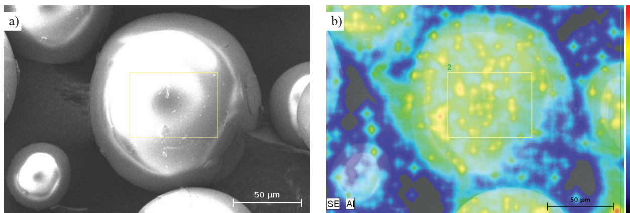
Fig. 10. a) SEM image of one of the microspheres chosen for thickness measurement after 200 cycles of \text{Al}_2\text{O}_3 deposition. The rectangular measurement area is indicated. b) Map of the intensity of EDS signal from Al measured in the same area. The average layer thickness determined for this sphere was 23.8 nm.
