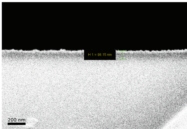
Fig. 15. Imaging with the mass contrast EsB detector shows that the AlN layer on a glass slide is ca. 100 nm-thick after 625 deposition cycles.
