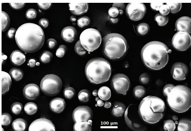
Fig. 5. Microspheres after depositing a 23 nm layer of \text{Al}_2\text{O}_3 . Despite being covered with a thin conductive layer (Au-Pd), the spheres accumulate some electric charge, which results in apparent shadows on the SEM image.
