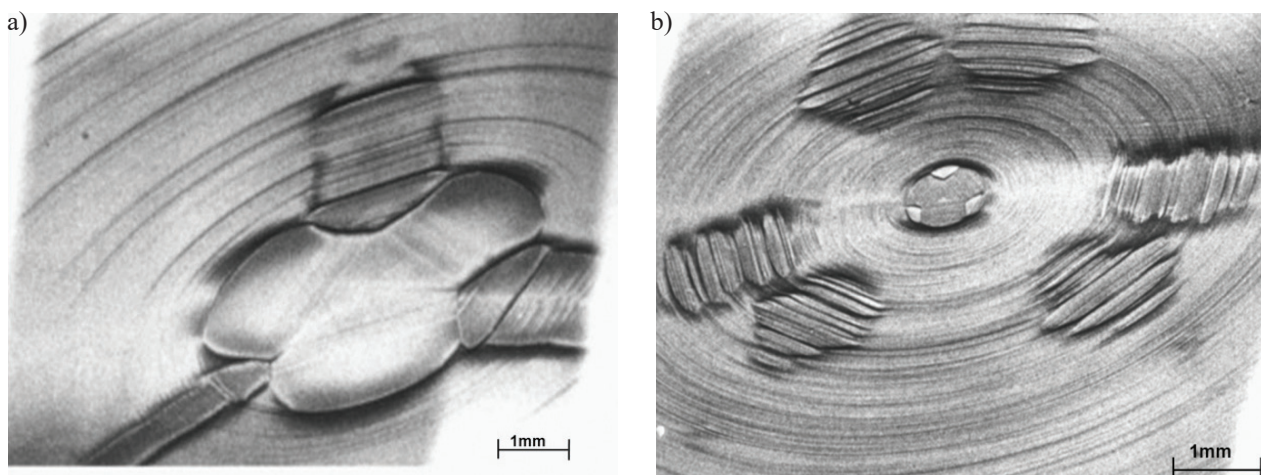
Fig. 8. White beam projection reflection topographs of Er-doped \text{Yb}_3\text{Al}_5\text{O}_{12} crystals revealing segregation fringes and sets of facets; doping level: (a) 10 at. % Er and (b) 1.5 at. % Er; (a) 422 reflection, 0.0872 nm radiation, (b) 112 reflection, 0.4 nm radiation. According to K. Kołodziejak et al. [66].
