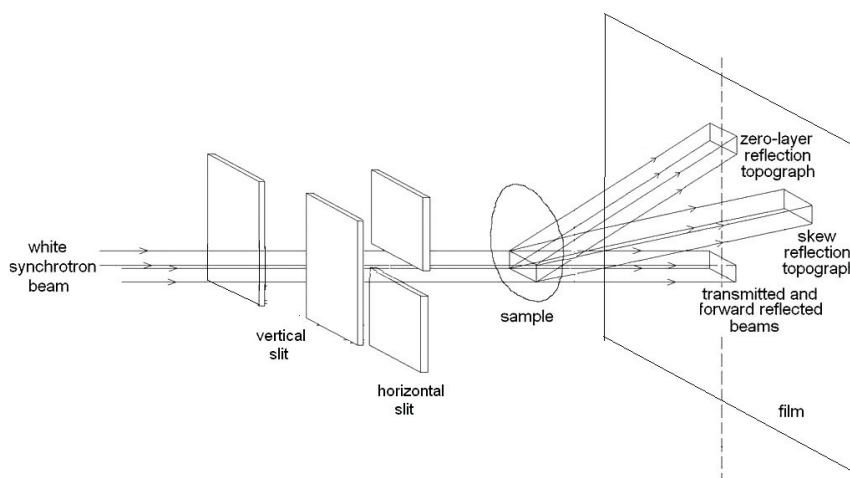
Fig. 3. The scheme of the synchrotron white beam topography in transmission case [57].
