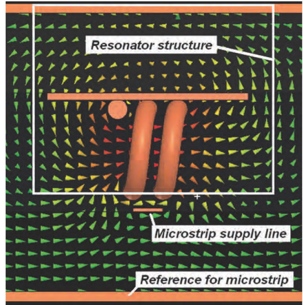
Fig. 6. Visualization of microwave magnetic field in resonator.
