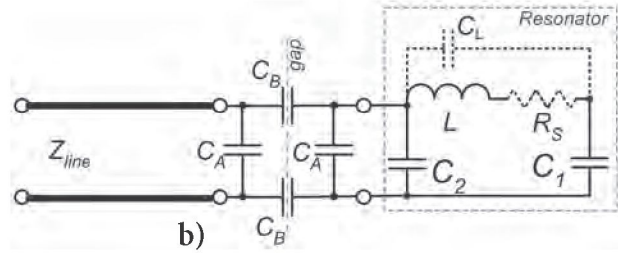
Fig. 3. Helix resonator electrically coupled with microstrip line: a) electrical coupling with the resonator; b) equivalent circuit diagram.
