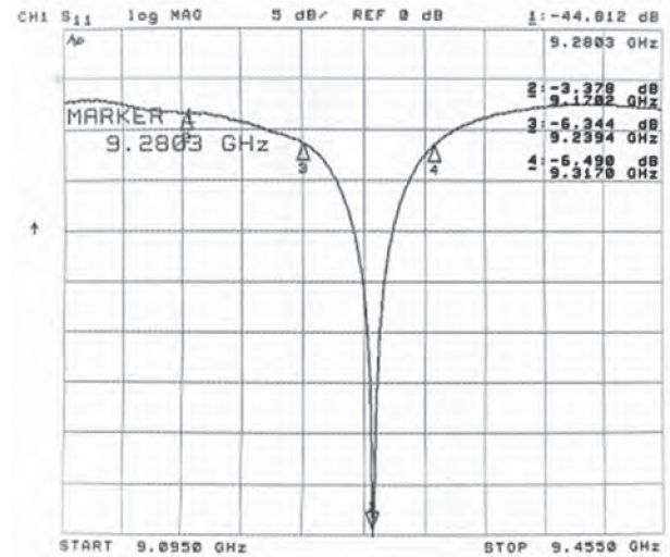
Fig. 7. Resonator response.
