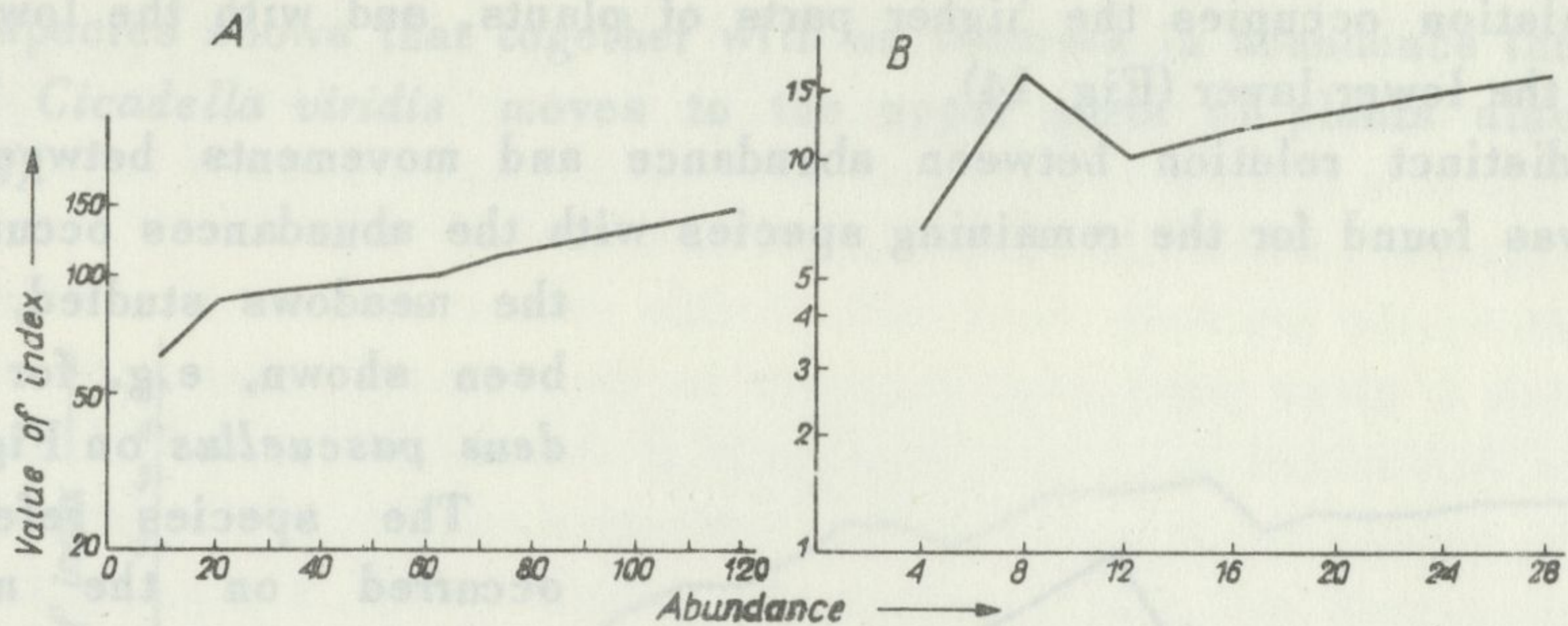
Fig. 12. Variations in value of index h for Neophilenus lineatus (A) and Philenus spumarius (B)
