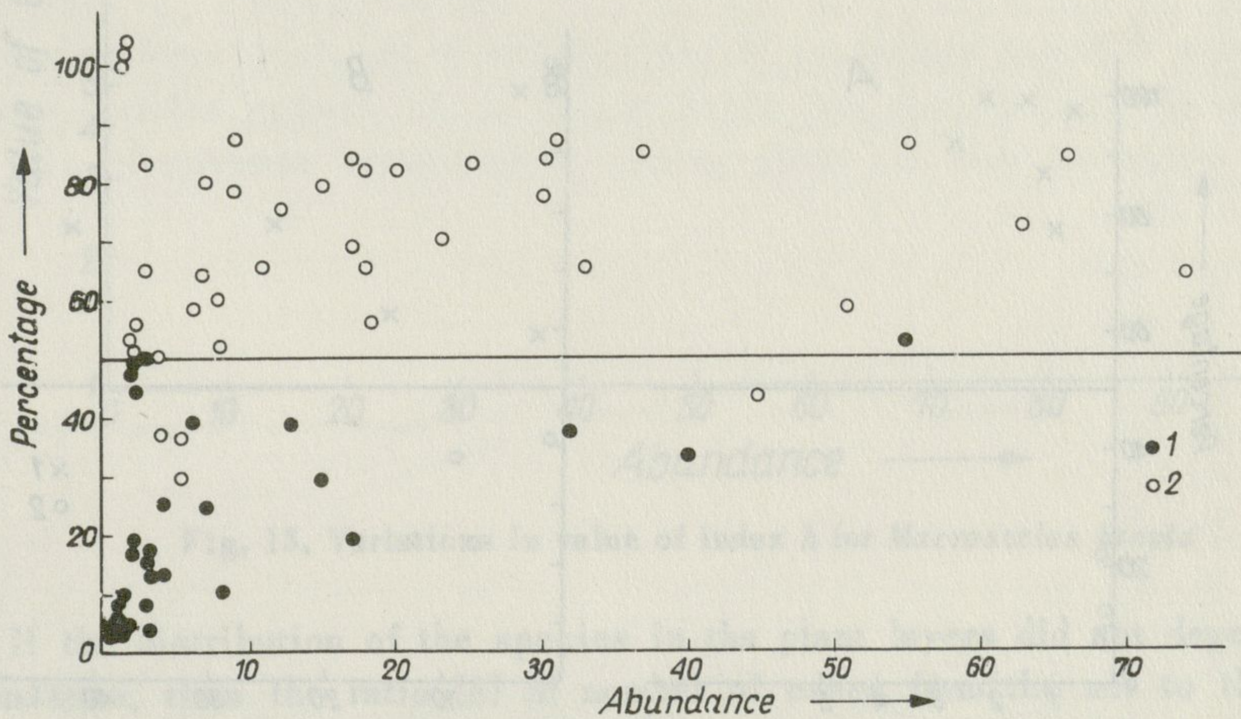
Fig. 9. Correlative comparison of abundance of the species Arthaldeus pascuellus with its percentage in the given layer
