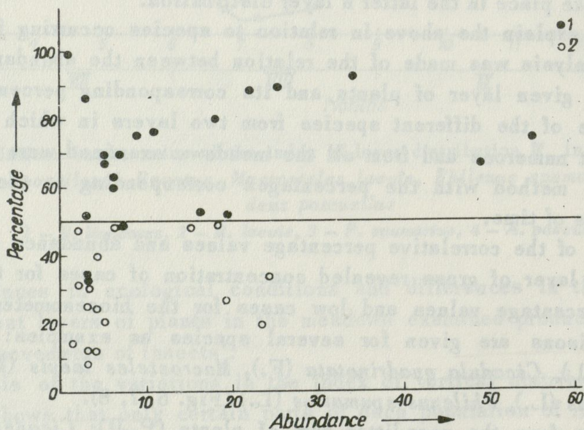
Fig. 7. Correlative comparison of abundance of the species Macrosteles laevis with its percentage in the given layer
