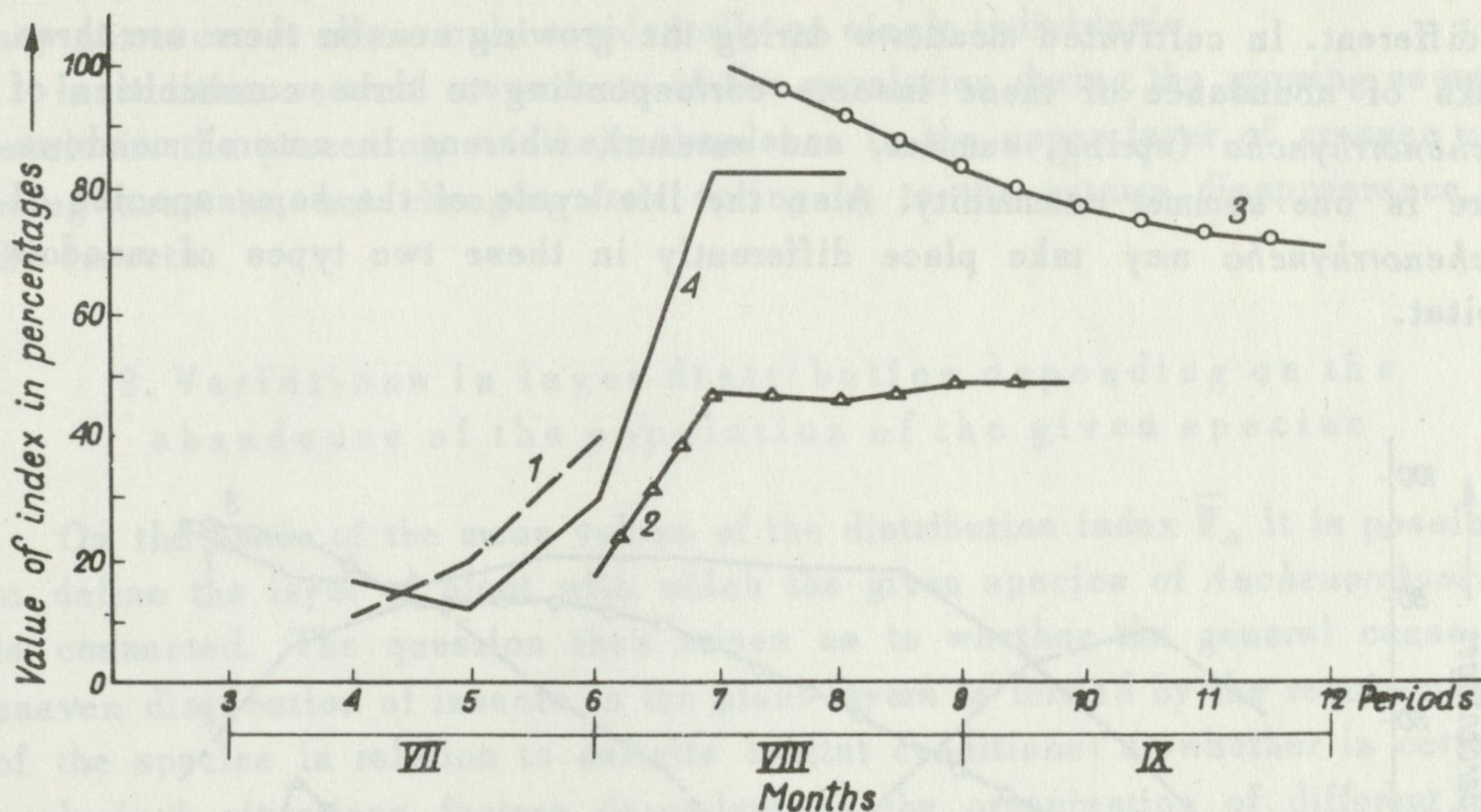
Fig. 3. Variations in the value of the index of layer distribution W_a in different periods of time for Arthaldeus pascuellus and Cicadula quadrinotata 1 - larvae A. pascuellus , 2 - imagines A. pascuellus , 3 - imagines C. quadrinotata , 4 - larvae C. quadrinotata
