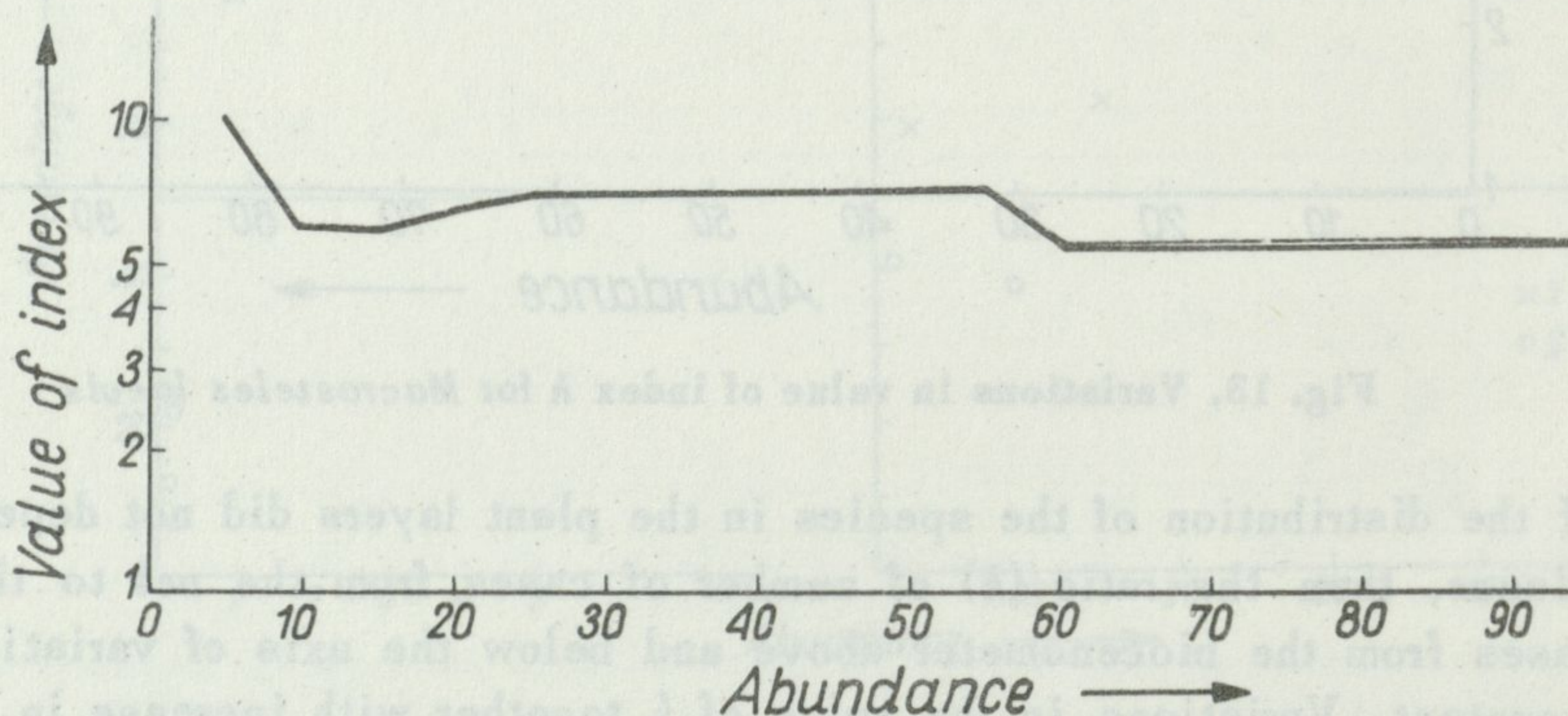
Fig. 15. Variations in value of index h for Arthaldeus pascuellus
