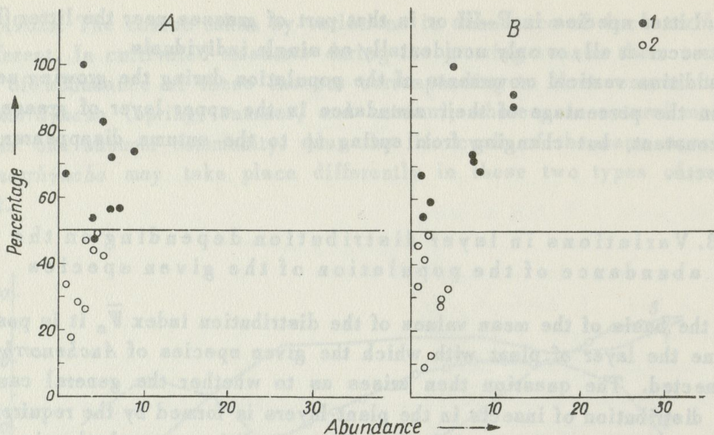
Fig. 6. Correlative comparison of abundance of the species Sorhoanus assimilis (A) and Cicadula quadrinotata (B) with their percentage in the given layer
