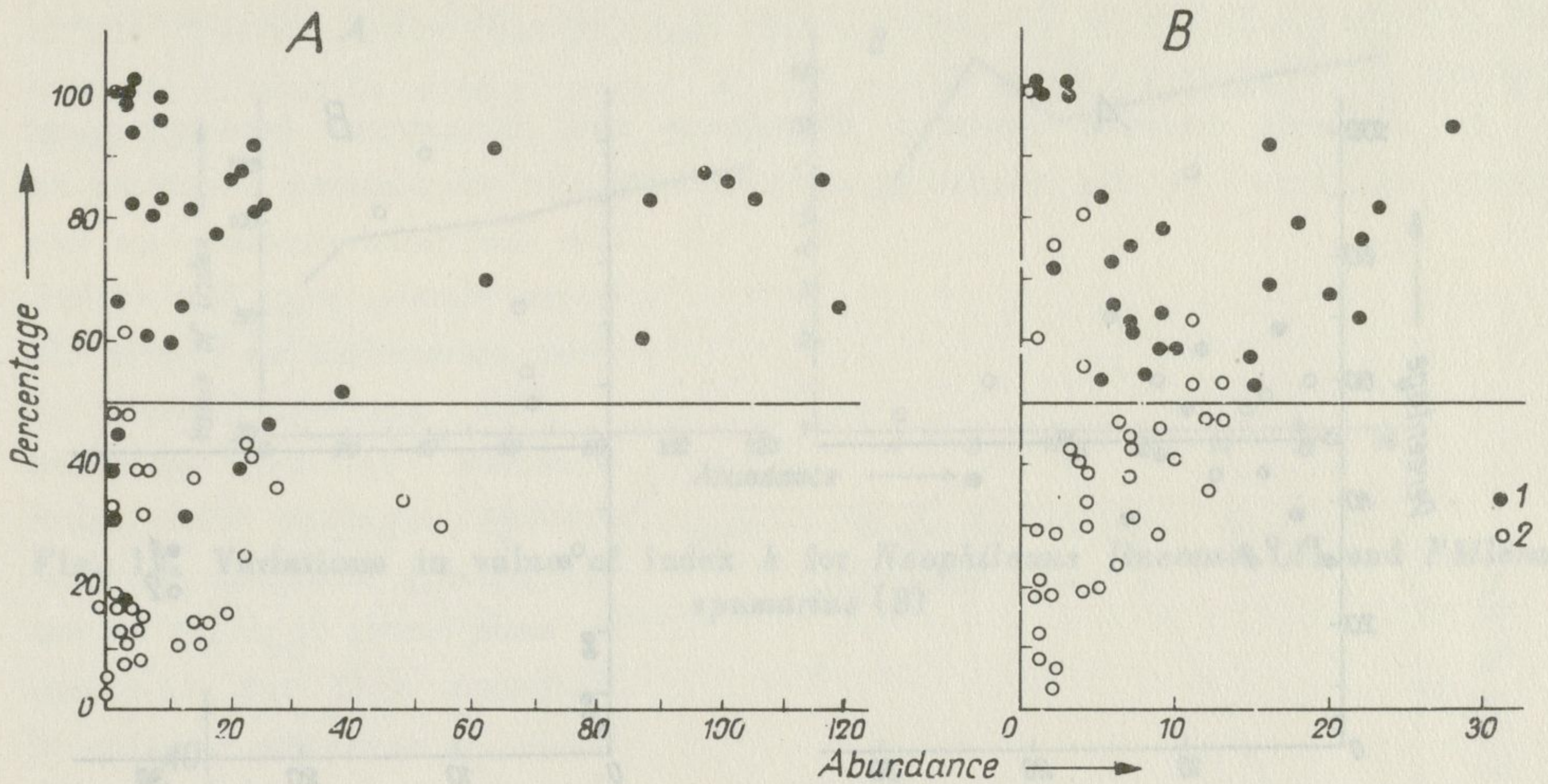
Fig. 8. Correlative comparison of abundance of the species Neophilenus lineatus (A) and Philenus spumarius (B) with their percentage in the given layer
