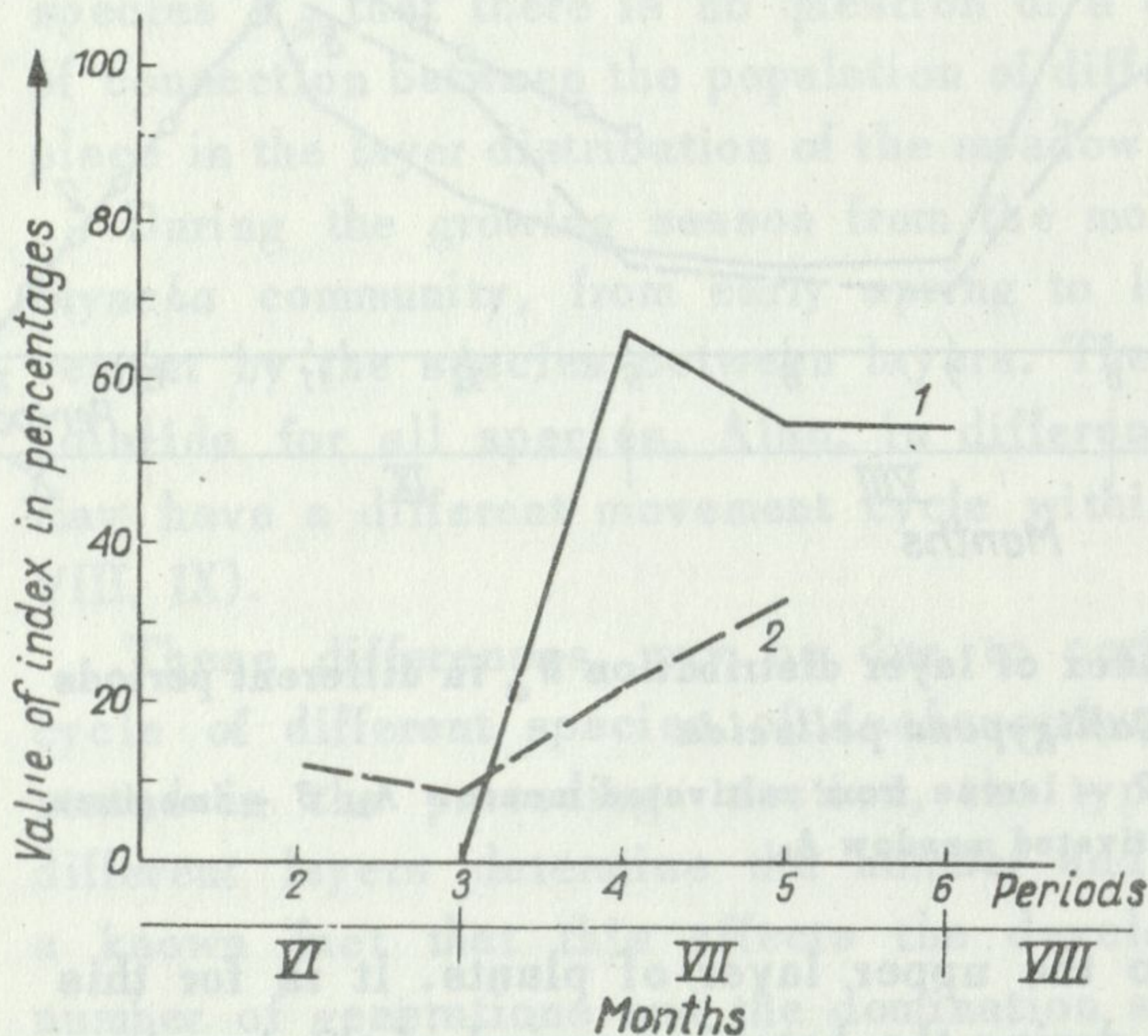
Fig. 2. Variations in the value of the index of layer distribution W_a in different periods of time for Cicadella viridis 1 – imagines, 2 – larvae
